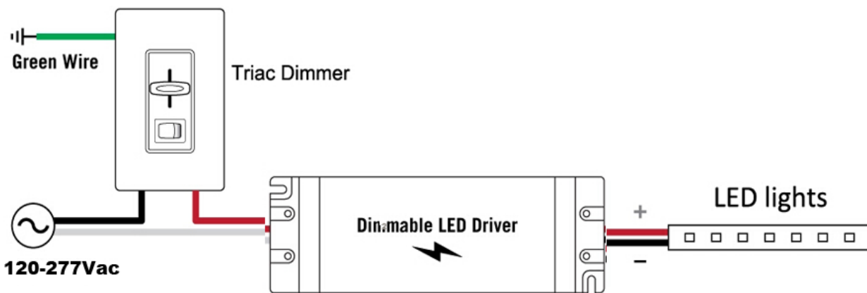
产品接线示意图/ Product Connection Diagram
